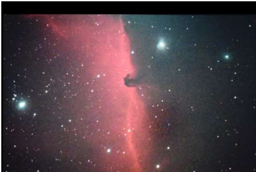
Horsehead Nebula
